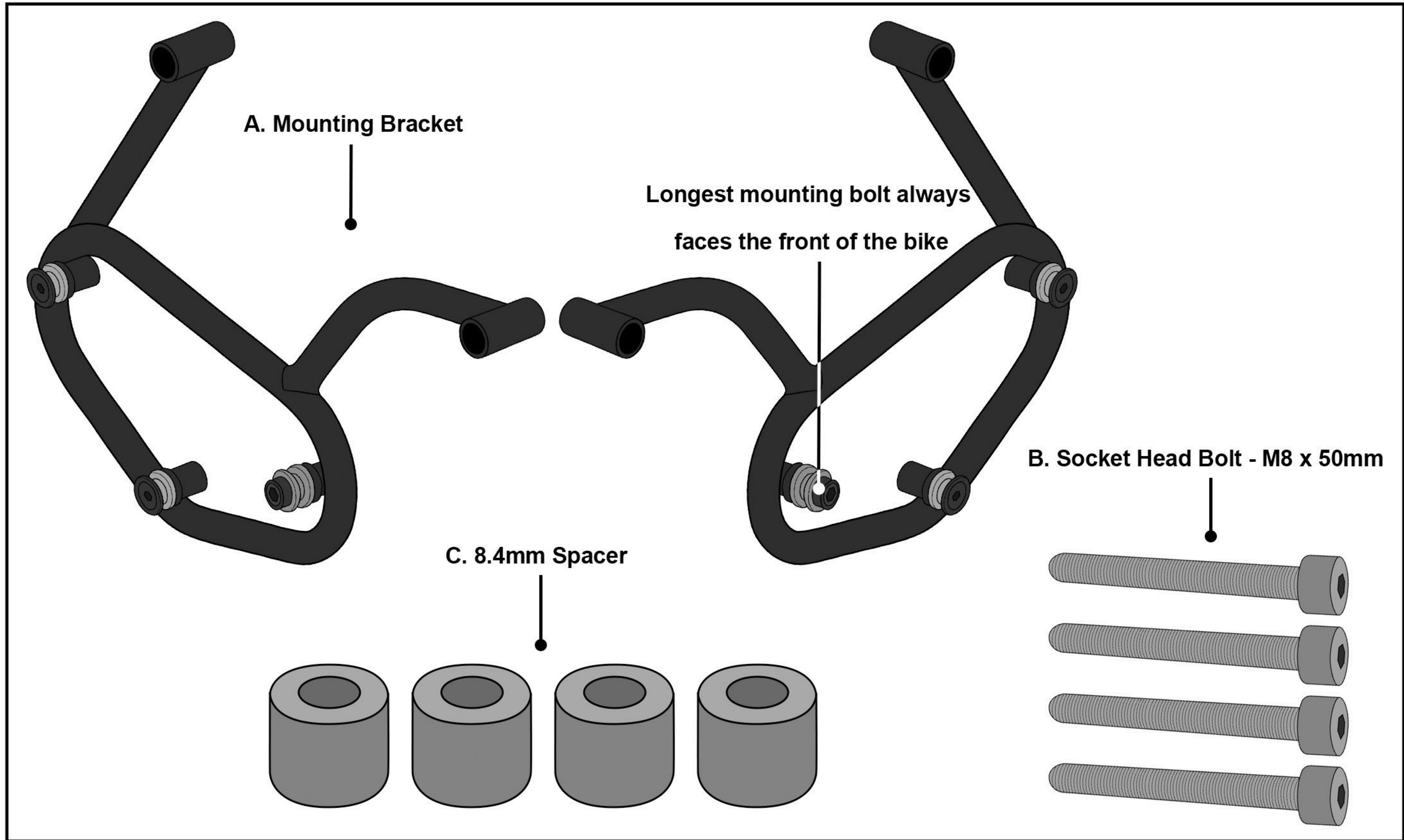
Parts Diagram
