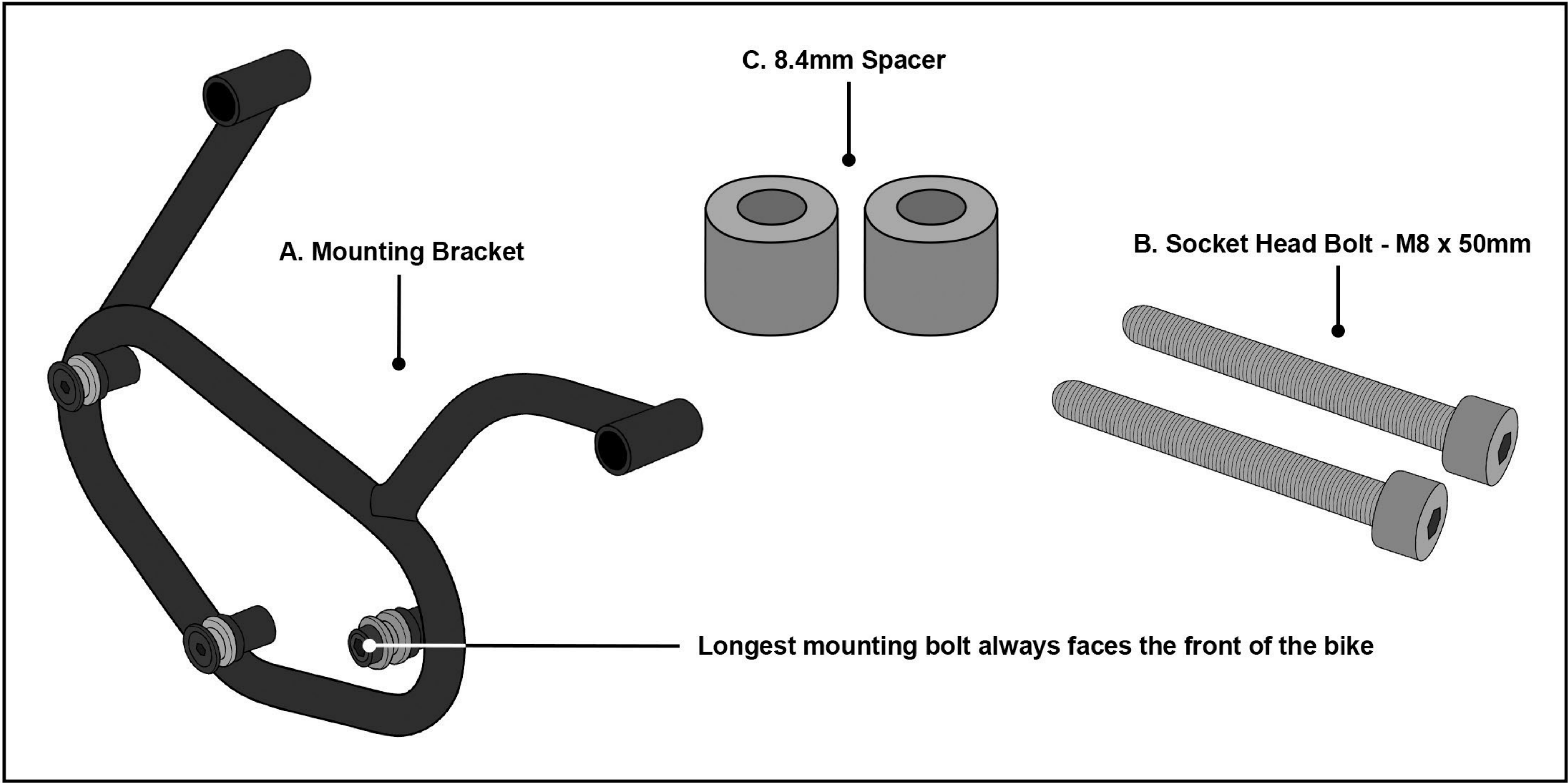
Parts Diagram
