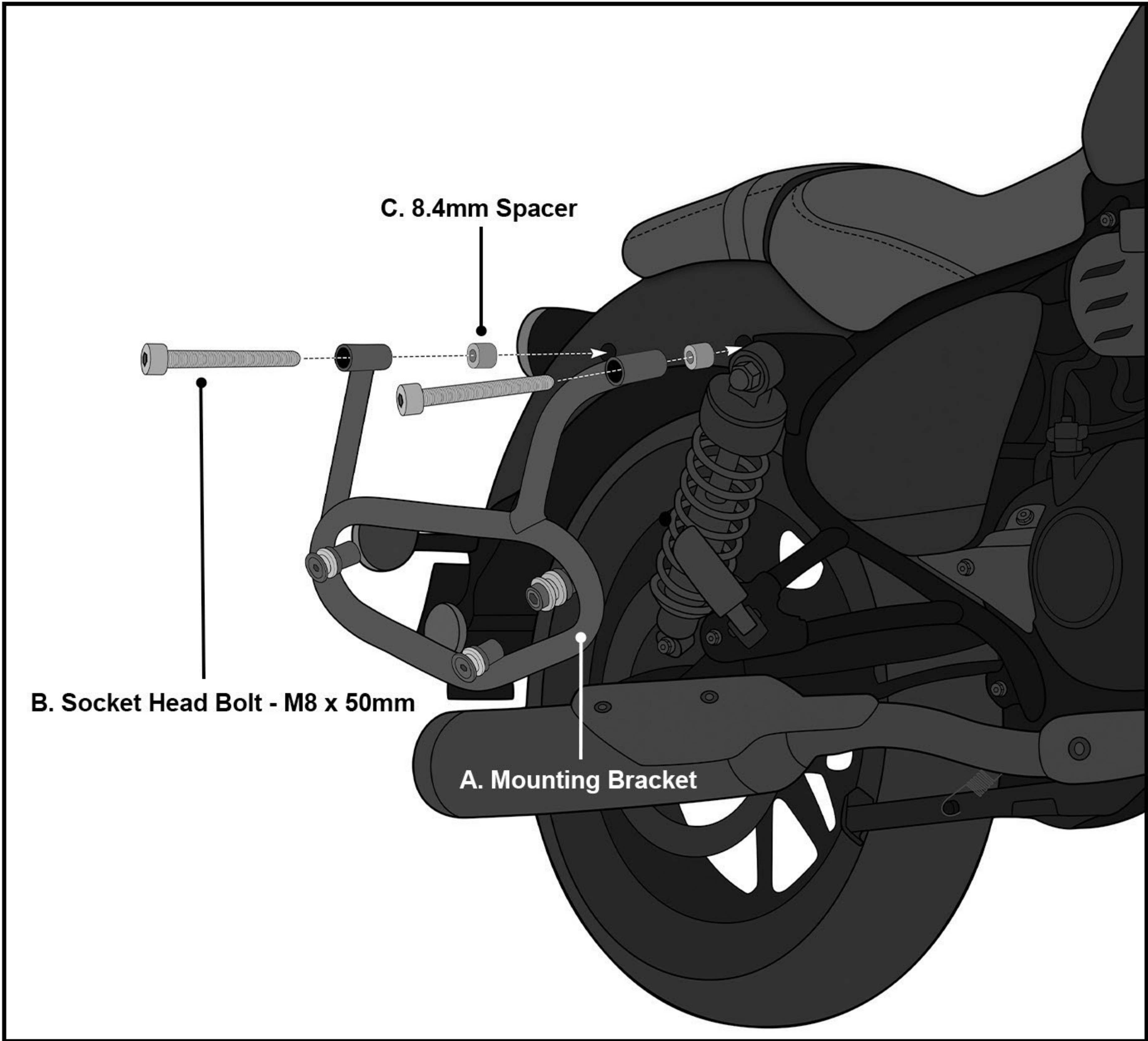
Fig 2. Attaching the Mounting Bracket
