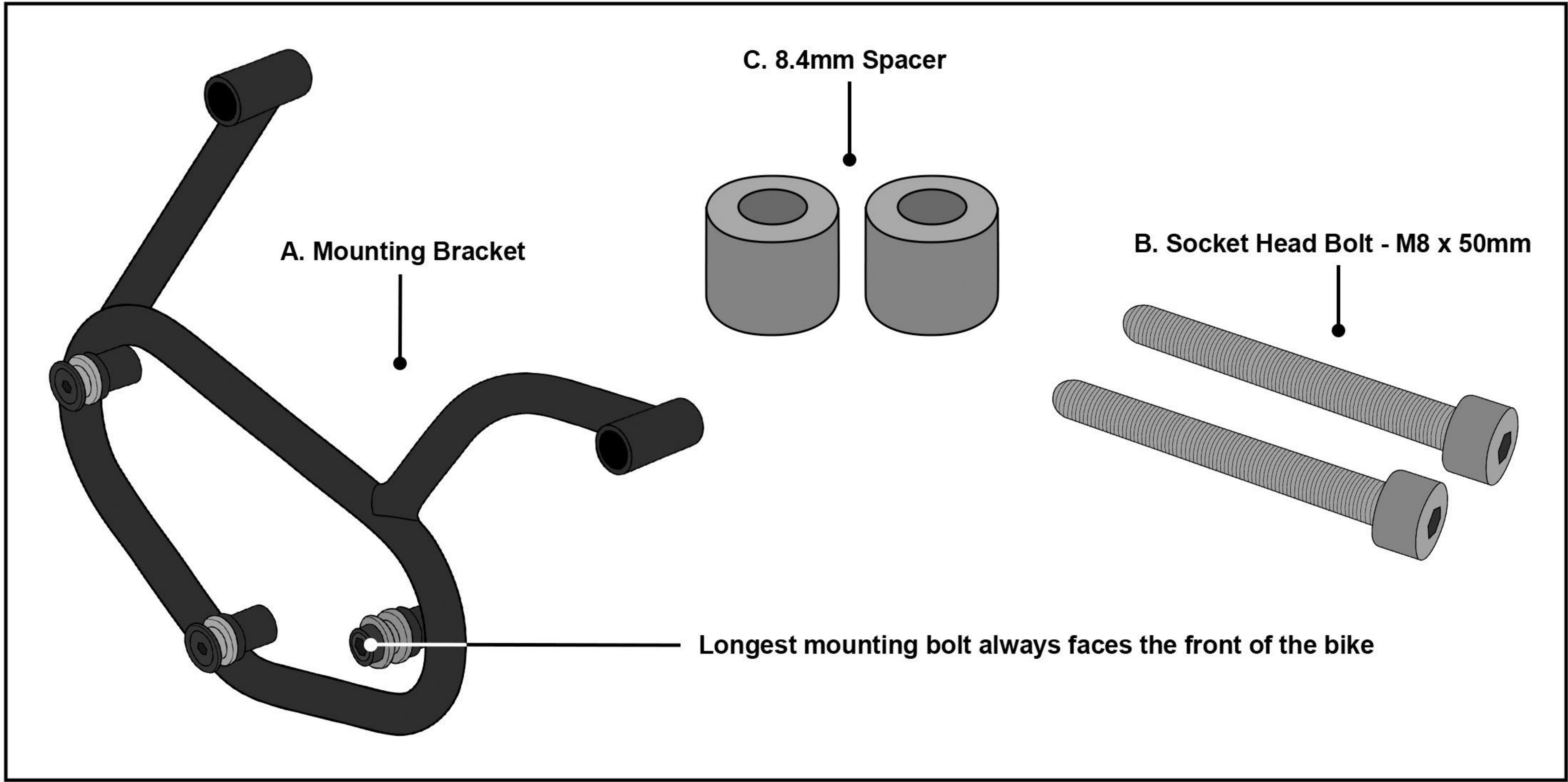
Parts Diagram
