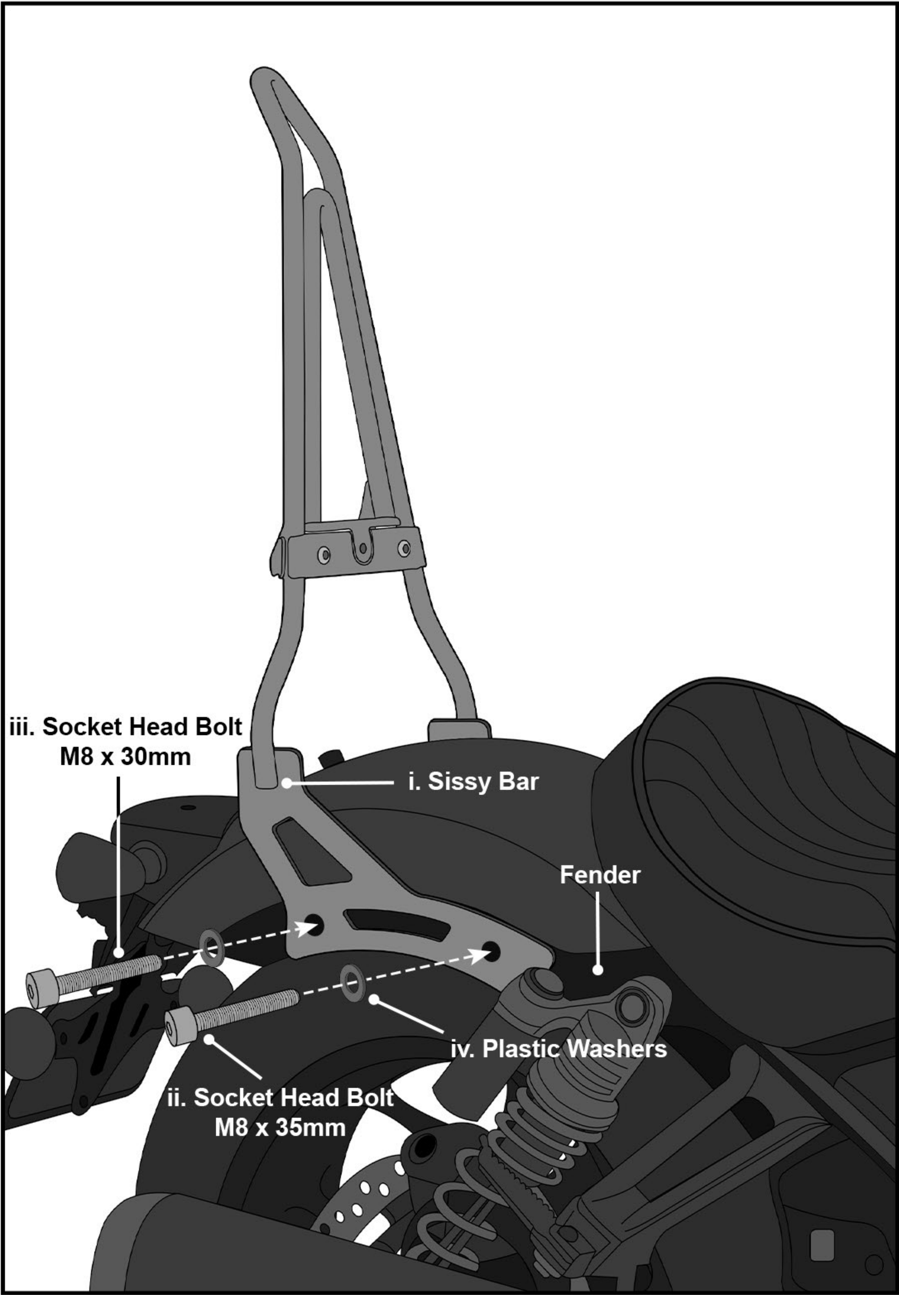
(Fig A) Sissy Bar Installed on Bike
