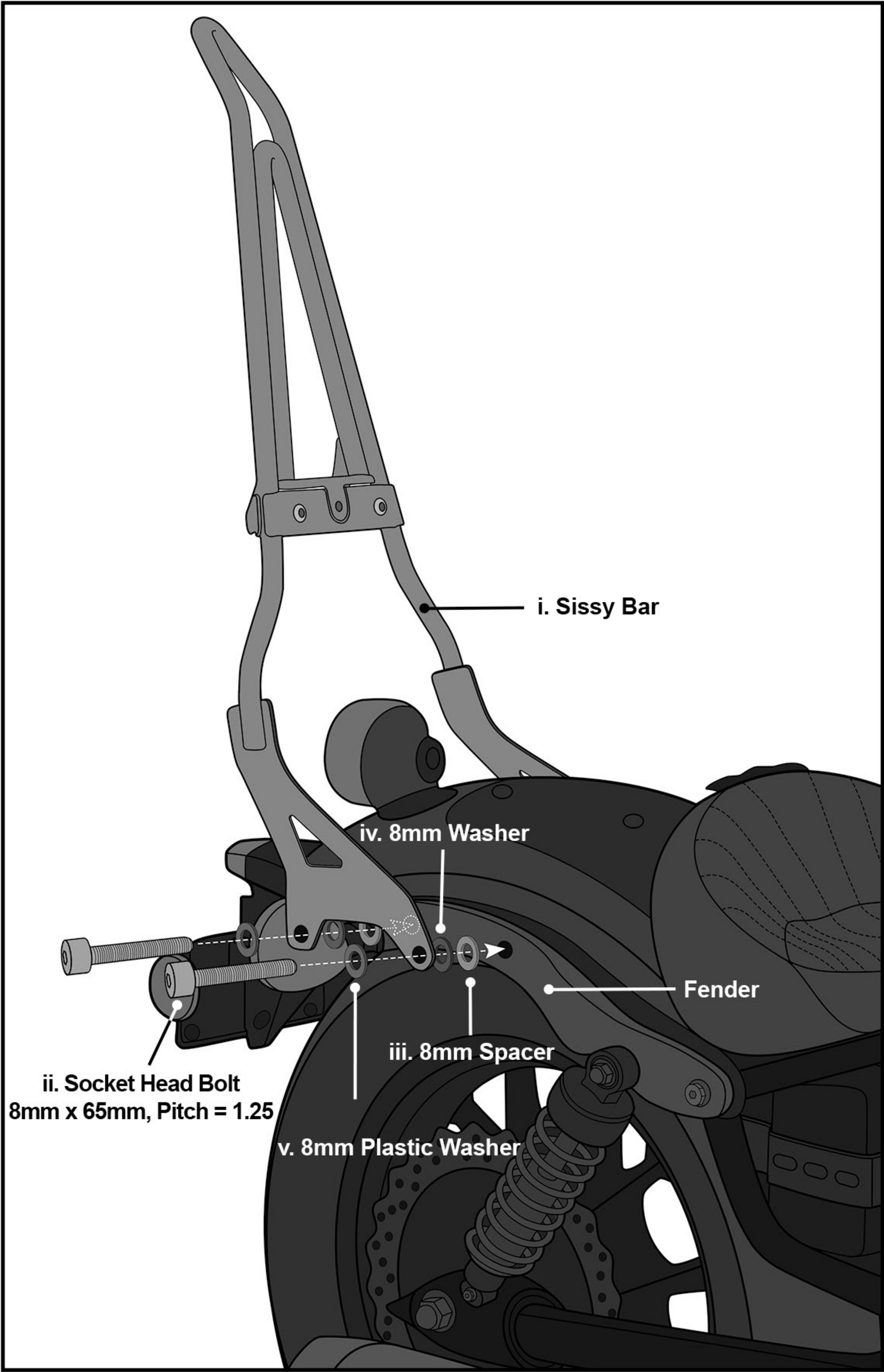
(Fig A) Sissy Bar Installed on Bike
