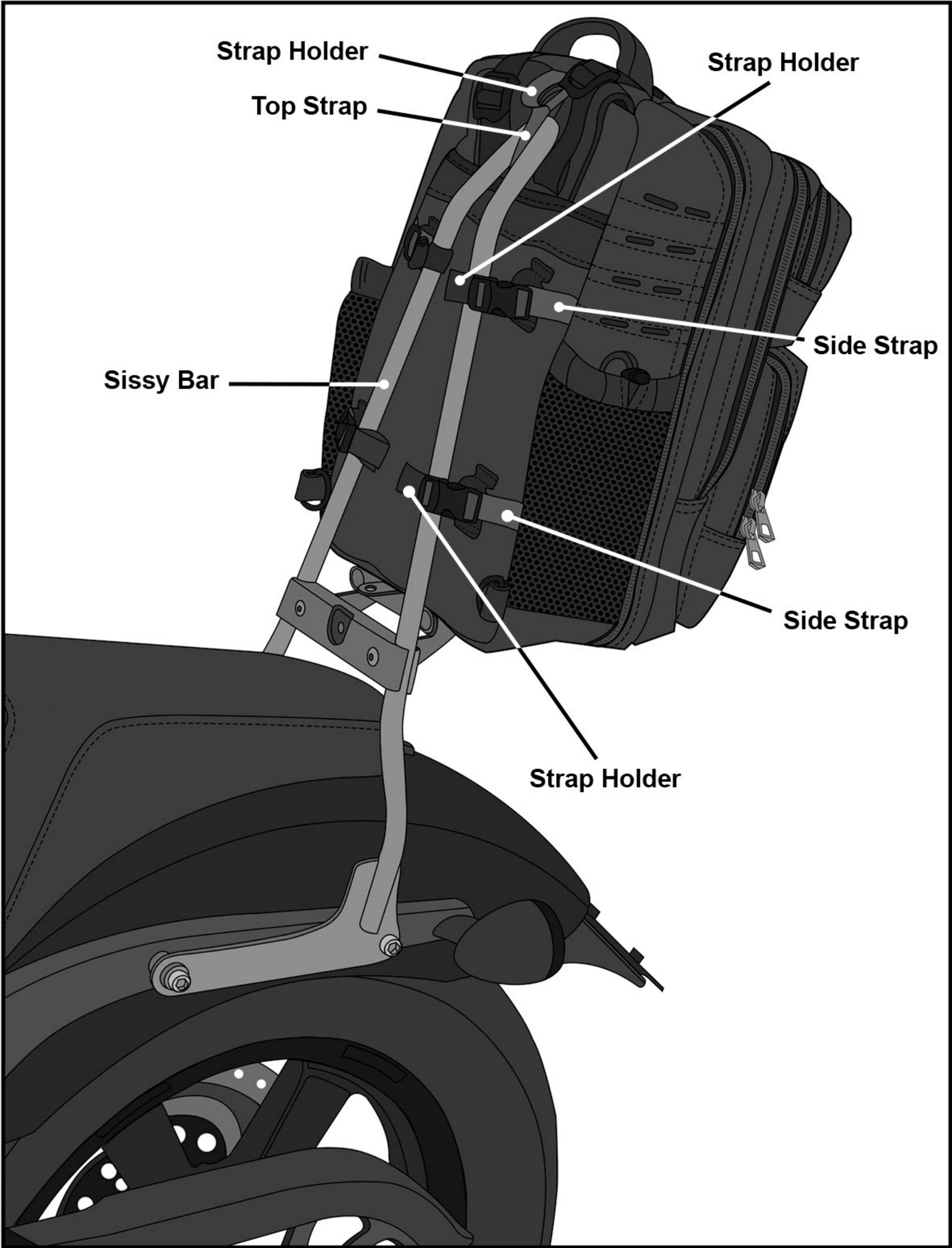
Fig (A) Bag Installed to Sissy Bar
